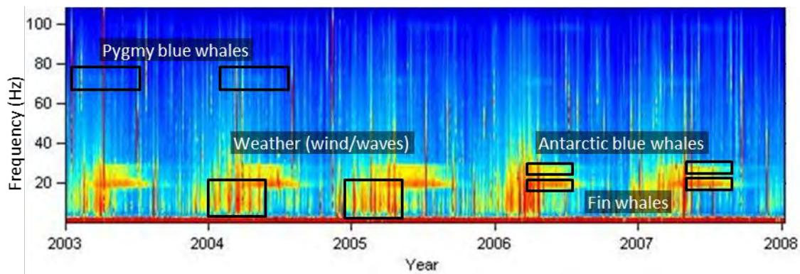
Figure 3-1. Long-term spectrogram (5 years) illustrating repetitive seasonal changes in the soundscape, due to weather, and singing Antarctic and pygmy blue, and fin whale populations south of Australia. Data is from the Comprehensive Nuclear Test Ban Treaty Organization (CTBTO) passive hydroacoustic monitoring station off Cape Leeuwin, Australia.
